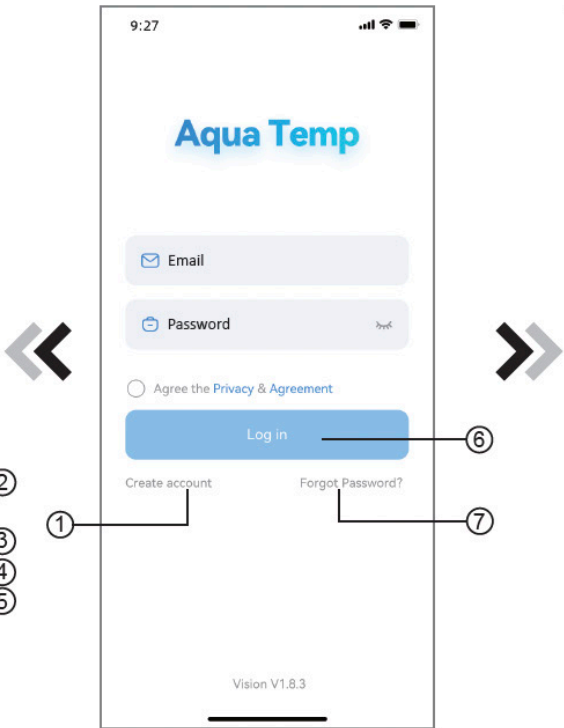
Fig.1 Login interface
