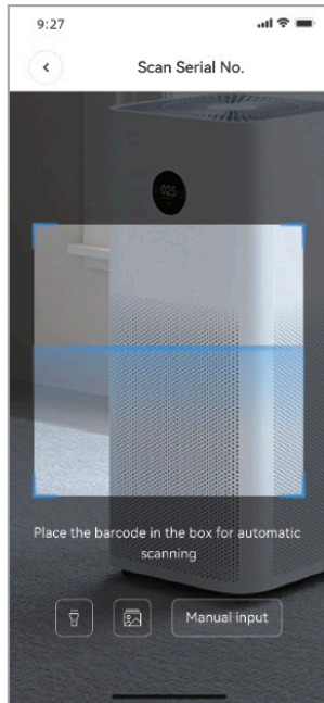
Fig.12 Scanning interface
