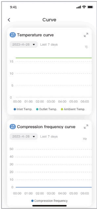
Fig.18 Curve interface
